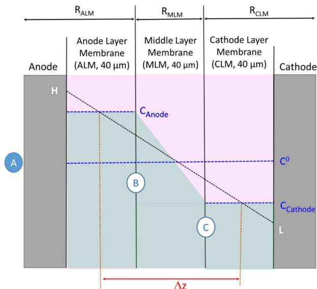
Figure 2. Sketch of the layered membrane cell, reference electrode configuration and the acid concentration profile. A and D are gas diffusion electrodes and B and C are reference electrodes. R_{\text{MLM}} is the measured resistance across the middle layer membrane (MLM) while R_{\text{ALM}} and R_{\text{CLM}} are the measured resistances of the anode layer membrane (ALM) and the cathode layer membrane (CLM), respectively, including the electrode layer. C^0 is the initial acid concentration through the three layer membrane. The black dashed line HL indicates the linear acid concentration gradient developed when a steady state between migration and diffusion is reached. The light blue profile is the model assumption where the anode ( C_{\text{Anode}} ) and cathode ( C_{\text{Cathode}} ) acid concentration are an average through the ALM and CLM, respectively, which drives the back diffusion across a distance of \Delta z .
